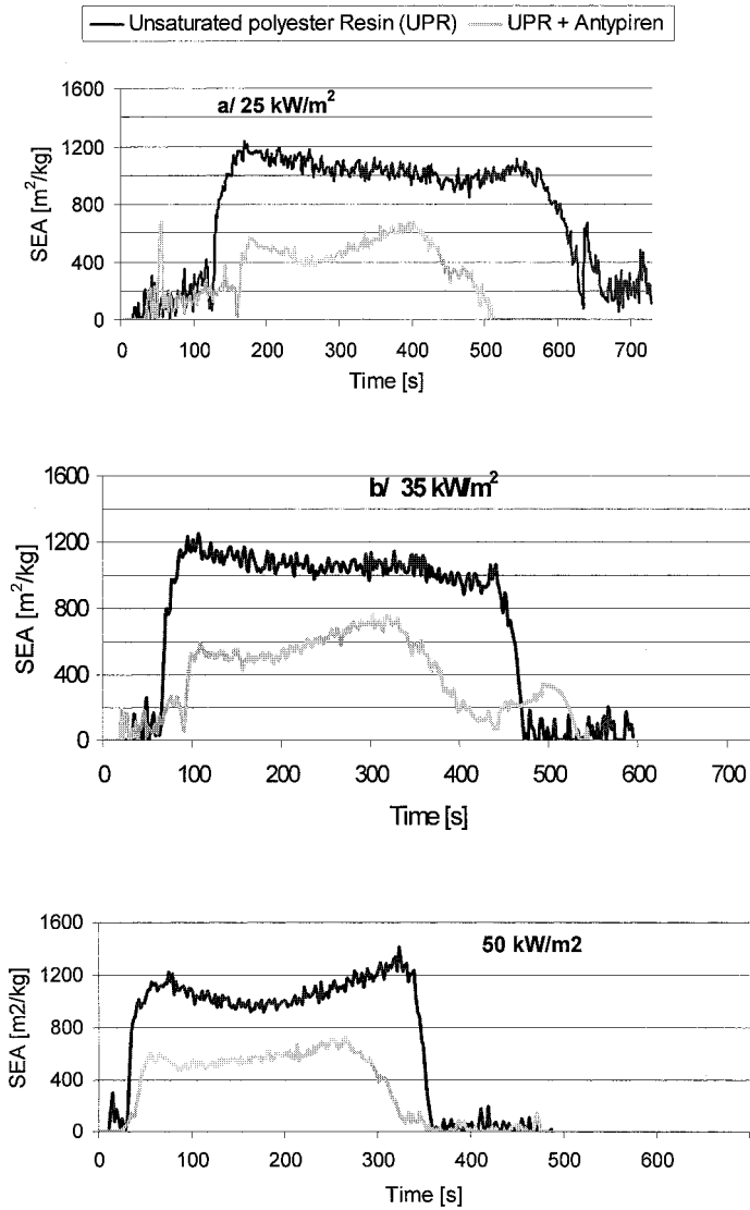
Fig. 6. The specific extinction area (SEA, \text{m}^2/\text{kg} ) of: 1 - fire-nonretarded, 2- fire-retarded GRP, in relation to thermal irradiation power: a - 25, b - 35, c - 50 \text{kW}/\text{m}^2 .
