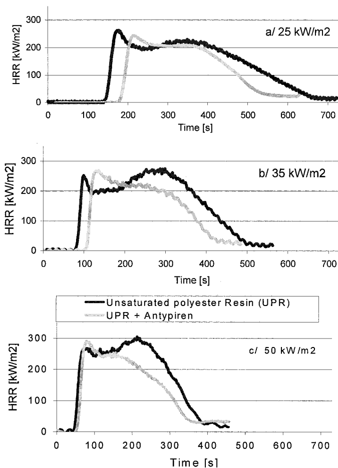
Fig. 1. The heat release rate (HRR) in relation to thermal irradiation power ( \text{kW/m}^2 ): a-25, b-35, c- 50; 1 - fire-nonretarded, 2- fire-retarded GRPL.
