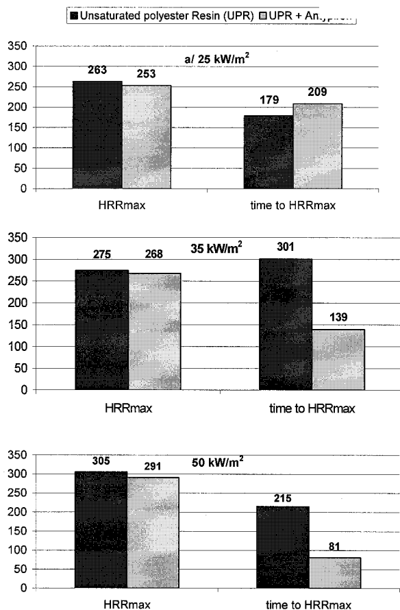
Fig. 3. The maximum HRR ( HRR_{max} ) and time required to attain HRR_{max} in relation to thermal irradiation power (for other designations see Fig. 1.).
