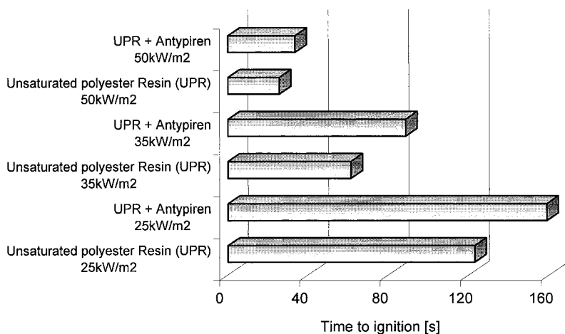
Fig. 4. Time required to ignite ( \tau_{ign} ) in relation to thermal irradiation power: 1 - fire-retarded, 2 - fire nonretarded GRP.
