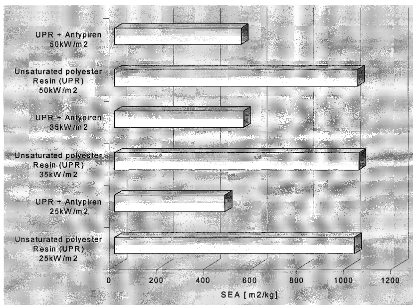
Fig. 7. The average extinction area ( SEA_{av} ) of: 1 - fire-nonretarded, 2 - fire-retarded GRP, in relation to thermal irradiation power indicated on ordinates.
