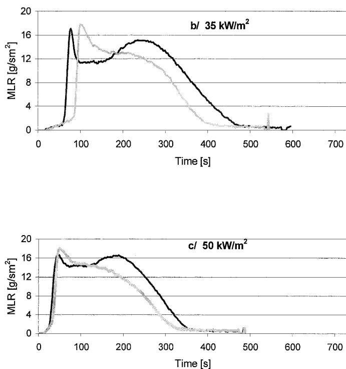
Fig. 8. The mass loss rate (MLR) in relation to thermal irradiation power: a - 25, b - 35, c - 50 \text{kW/m}^2 ( for other designations see Fig. 6).
