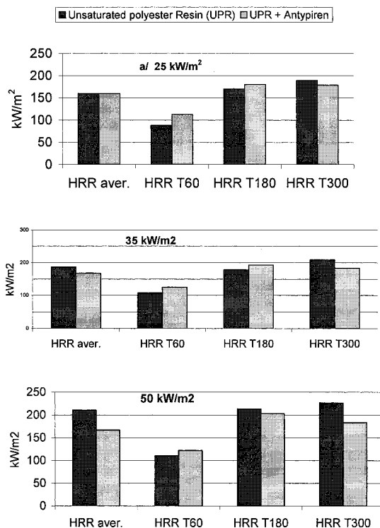
Fig. 2. The average HRR ( \text{HRR}_{\text{av}} ) and the HRR at the 60 th , 180 th and 300 th second reckoned from ignition in relation to thermal irradiation power (for other designations see Fig. 1).
