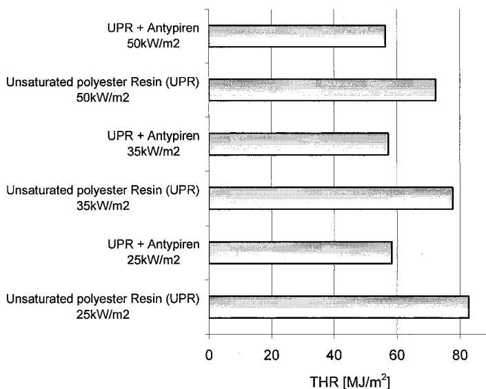
Fig. 5. Total heat released (THR) by: 1 - fire retarded, 2 - fire-nonretarded GRP in relation to thermal irradiation power.
